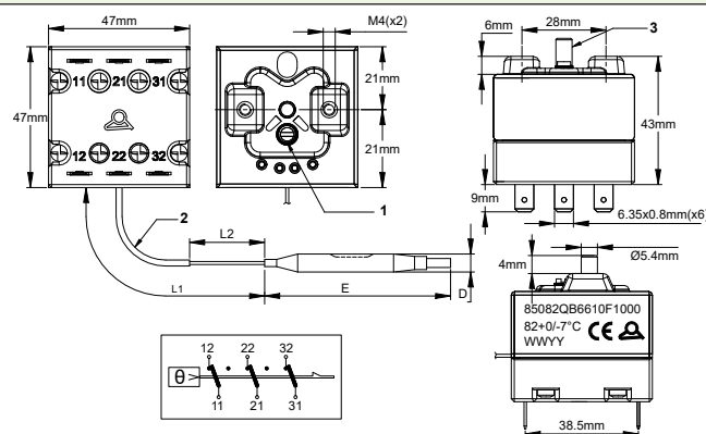
1. Sealing; 2. Sleeve; 3. Manual reset button
